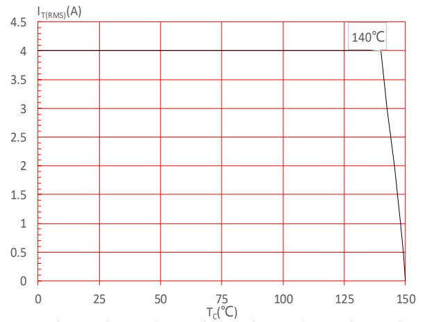
FIG.4: On-state characteristics
