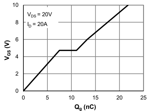
Gate Charge
